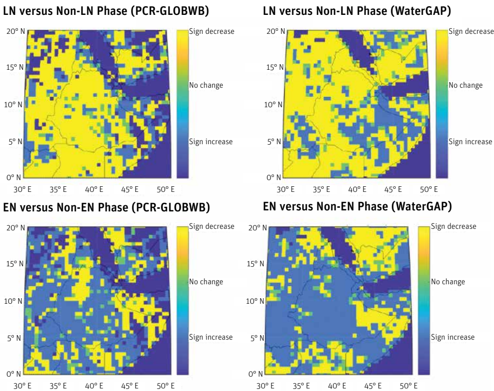
FIGURE 5.12 Spatial Distribution of Area with a Significant Increase, Decrease, or No Change in Frequency of Drought Months: El Niño Years Compared with Non–El Niño Years and La Niña Years Compared with Non–La Niña Years
