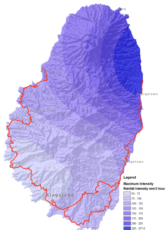
FIGURE 4: PRECIPITATION DISTRIBUTION
