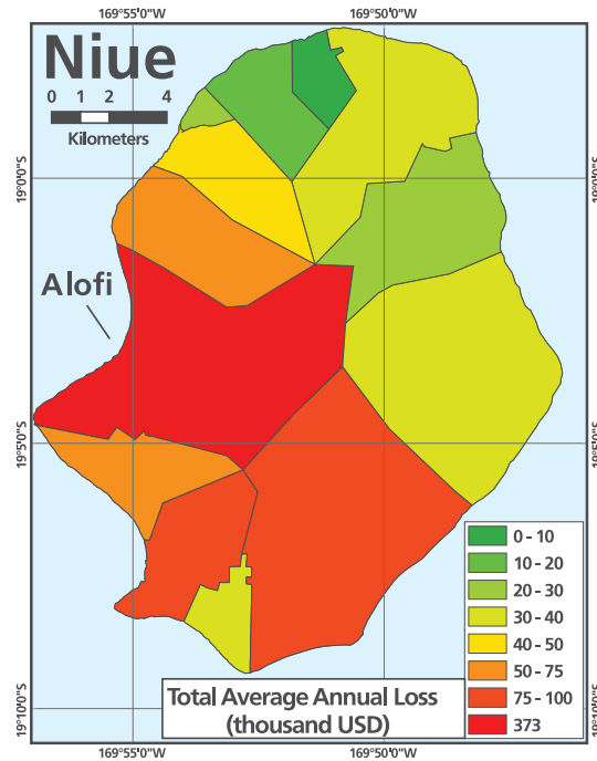
Figure 7: Contribution from the different villages to the average annual loss for tropical cyclone and earthquake (ground shaking and tsunami).
