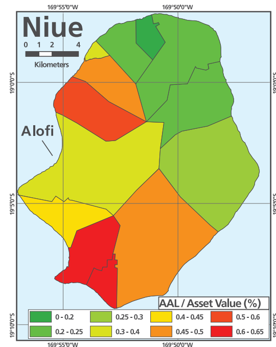
Figure 8: Contribution from the different villages to the tropical cyclone and earthquake (ground shaking and tsunami) average annual loss divided by the replacement cost of the assets in each village.
