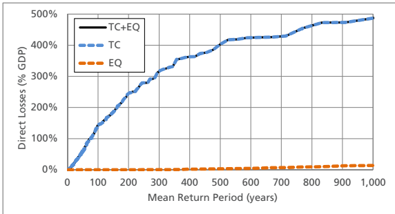
Figure 10: Direct losses (in absolute terms and normalized by GDP) caused by either tropical storms or earthquakes that are expected to be exceeded, on average, once in the time period indicated.
