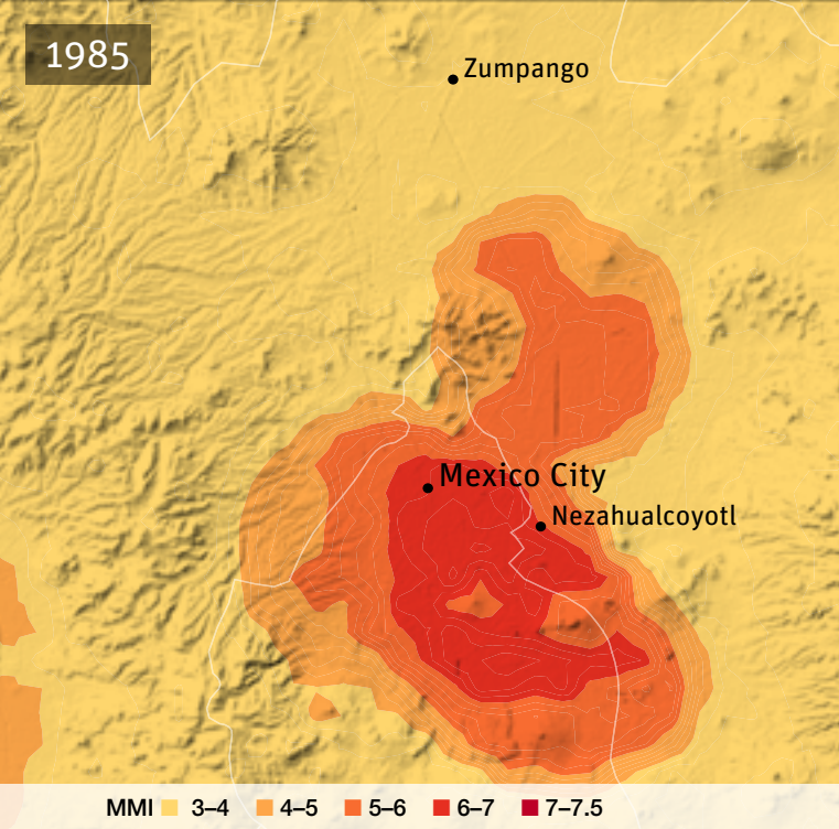
Shake maps showing the relative ground motions in terms of Modified Mercalli Intensity (MMI). Maps: USGS and Axis Maps
