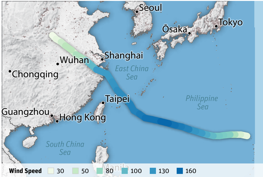
Track of Typhoon Wanda, 1956, showing wind speed in knots. Map: IBTrACS, Axis Maps
