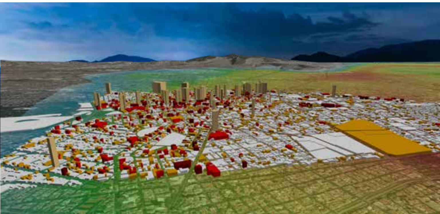
Expected damage (white, low damage; red, high damage) in downtown Mexico City due to a Mw 8.0 earthquake in the subduction zone. Ground motion is also shown (low intensity in blue, high intensity in red). Image: ERN
